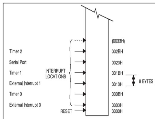
Fig. 3: Program Memory
