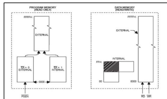
Fig. 3: Program Memory
