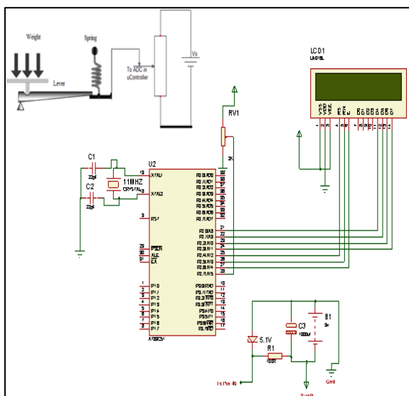
Fig. 7: The Circuit Diagram of the System
