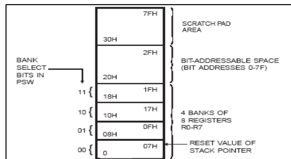
Fig. 6: The Lower 128 Bytes of Internal RAM
