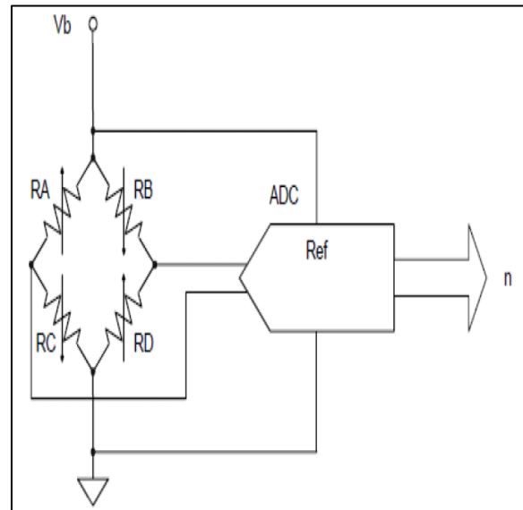
Fig. 8: Ratio-Metric Measurement
