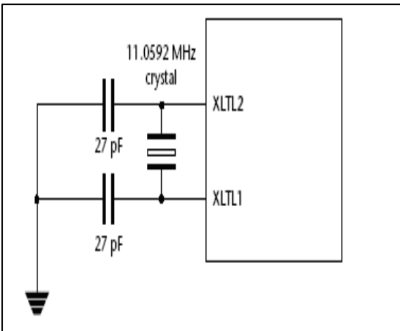
Fig 10: The Microcontroller Clock Input
