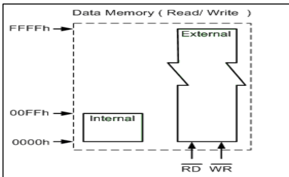
Fig 4: Data Memory Structure
