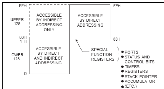
Fig. 5: Internal Data Memory
